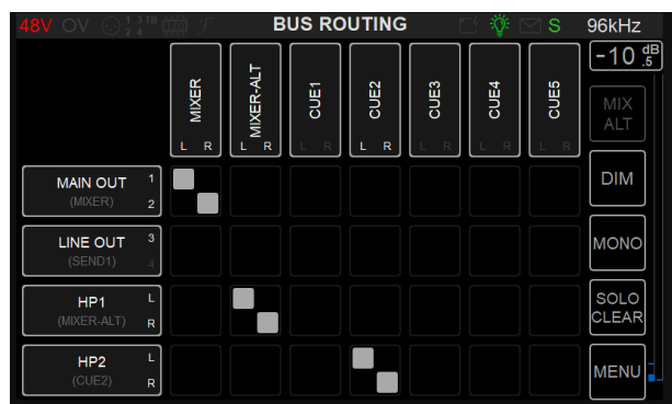
New Bus Routing (Firmware 1.2.5 and higher)
