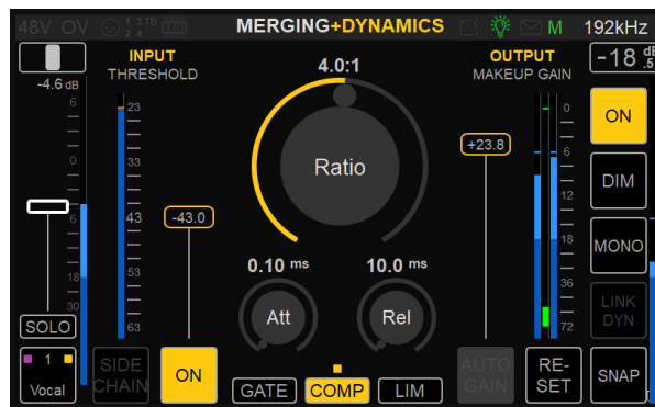
MERGING+DYNAMICS view
